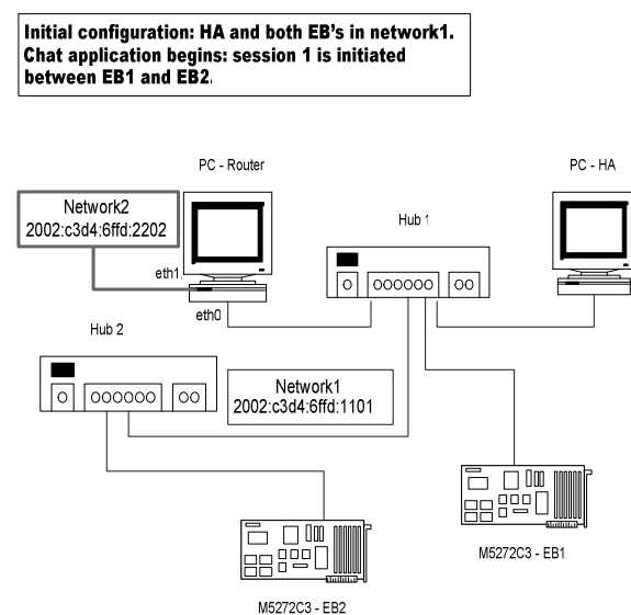
Figure 2 - Testbed
