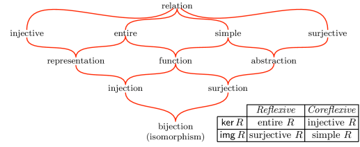
Figure 3: Binary relation taxonomy
