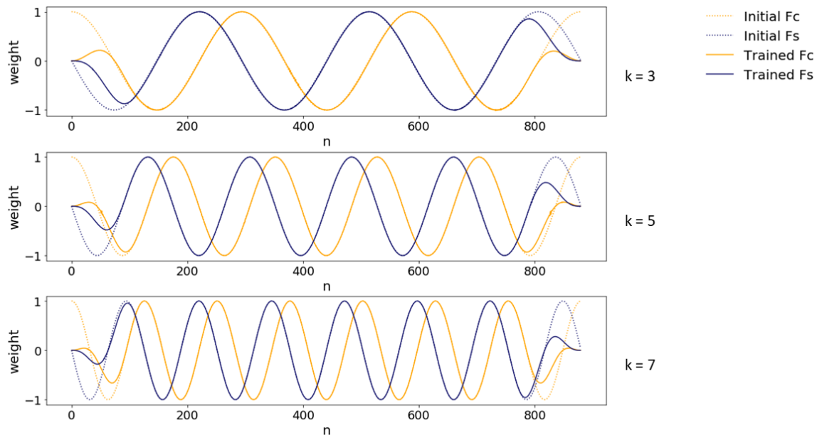
Figure 6: Trained weights vs. initial weights for case CL1-W in model III.
