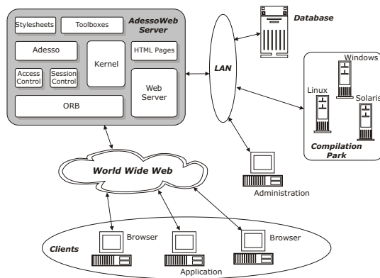
Fig. 5. AdessoWeb Organization
